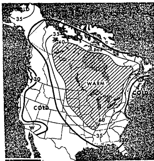
TEMPERATURE PROBABILITIES
